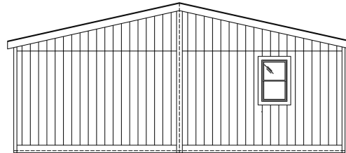
REAR ENDWALL
